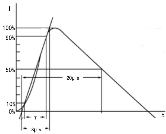
Fig Based on IEC61000-4-5 8/20 \mu s pulse.(Ed.2)
